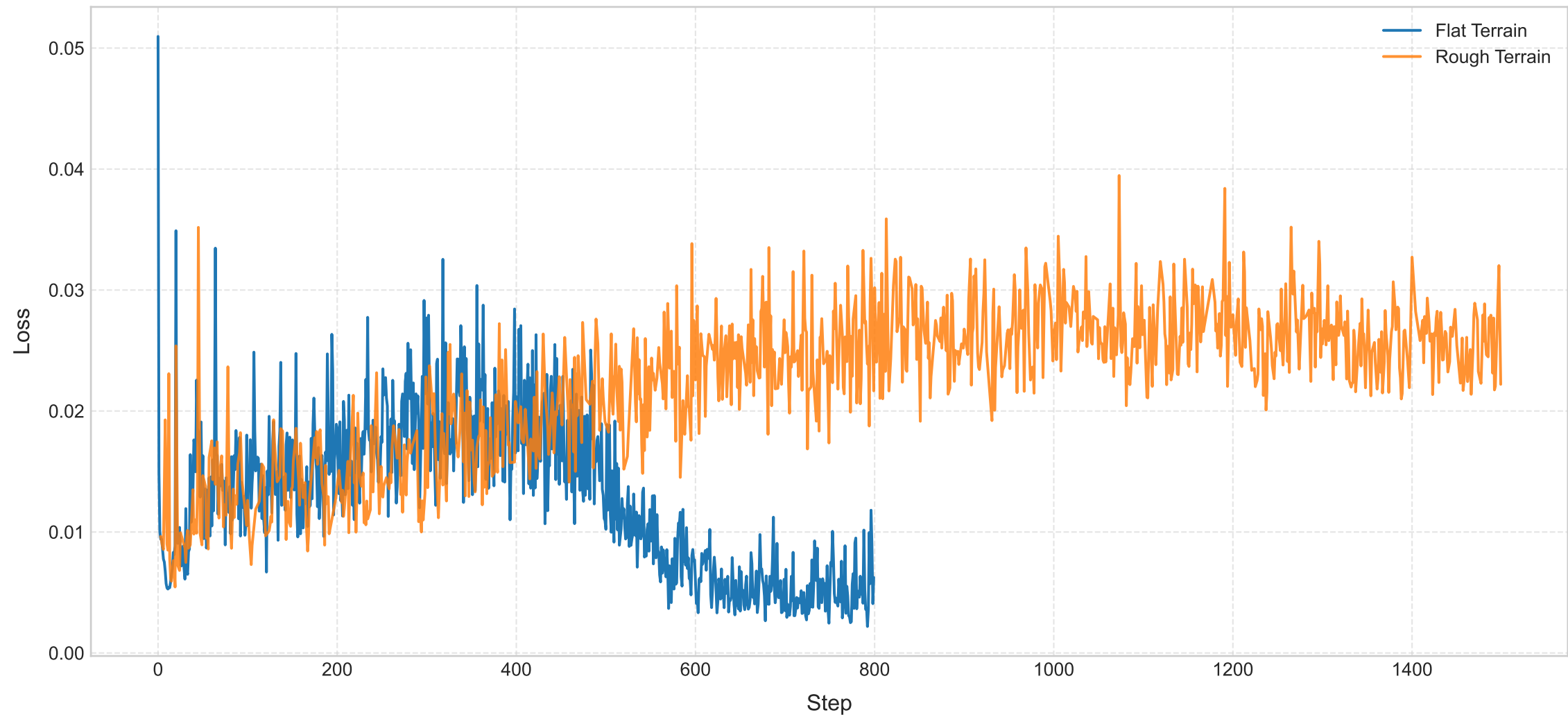
PPO Value Function Loss
